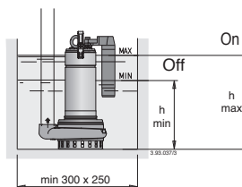
6.5.1. Stationary installation with vertical magnetic float switch
